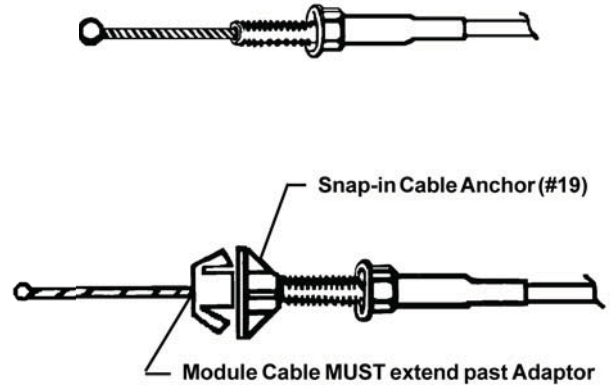
FIG. 11 THREADED SNAP-IN ADAPTOR
