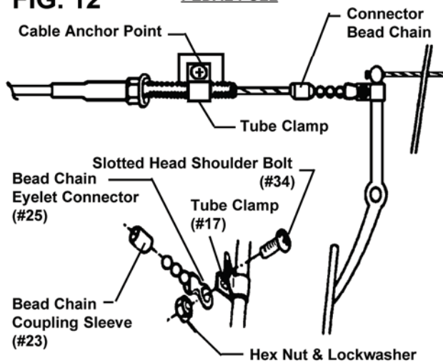
FIG. 12 PEDAL PULL
