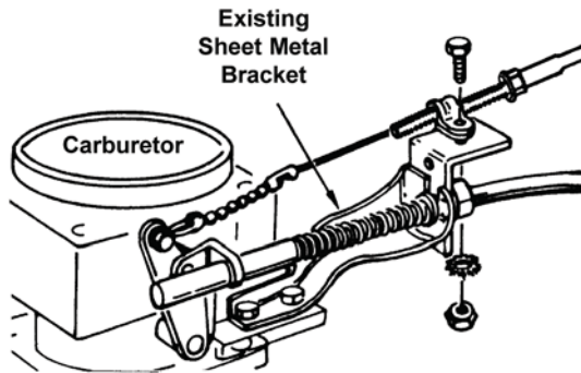
FIG. 12 PEDAL PULL
